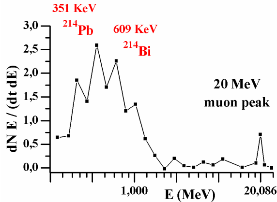
FIGURE 4. Energy spectrum obtained from the device
