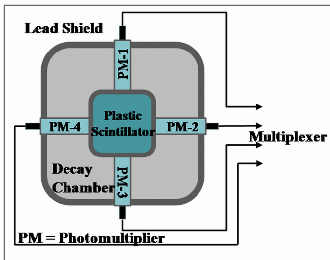
FIGURE 3. PM-4 detector section scheme
