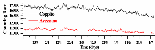
FIGURE 6. Raw data from Coppito and Avezzano stations (March-June 2004)
