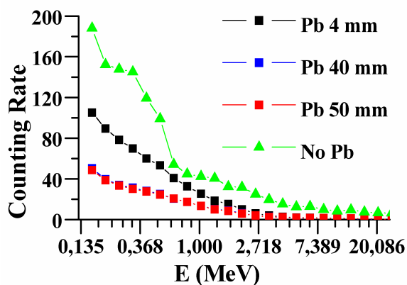
FIGURE 5. Effect of lead thickness on Rn measurements
