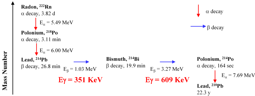
FIGURE 1. Decay chain about Radon
