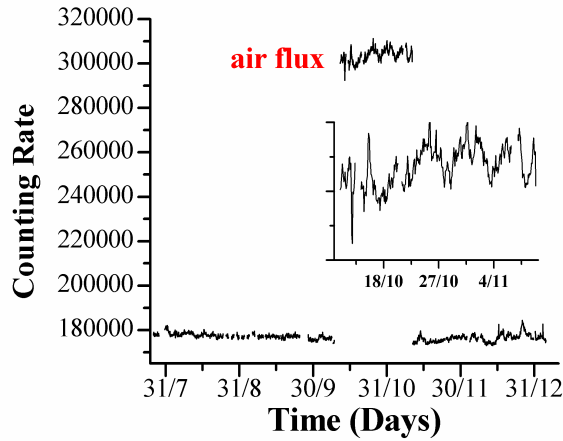
FIGURE 8. Test with air flux (July-December 2004)
