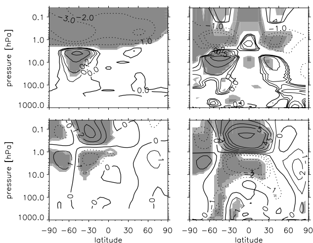
Fig. 2. Zonal mean difference between the regional (mid latitude 1hPa region) 20% ozone perturbations and the control experiments for the SMM (left) and for the ARPGE GCM (right). The responses in temperature (K – top) and zonal winds (m/s – bottom) are shown. Statistically significant changes at 99% level are shaded in grey (95% light grey).
