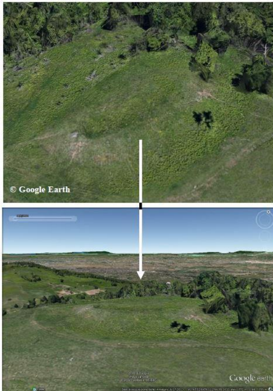
Fig. 1 – Three-dimensional model of the hill of Mount Salomone, in which the two walls, created by digging the ground, can be observed very well. In this case, the anthropic origin of the structure is clear. Credits: Google Earth.
